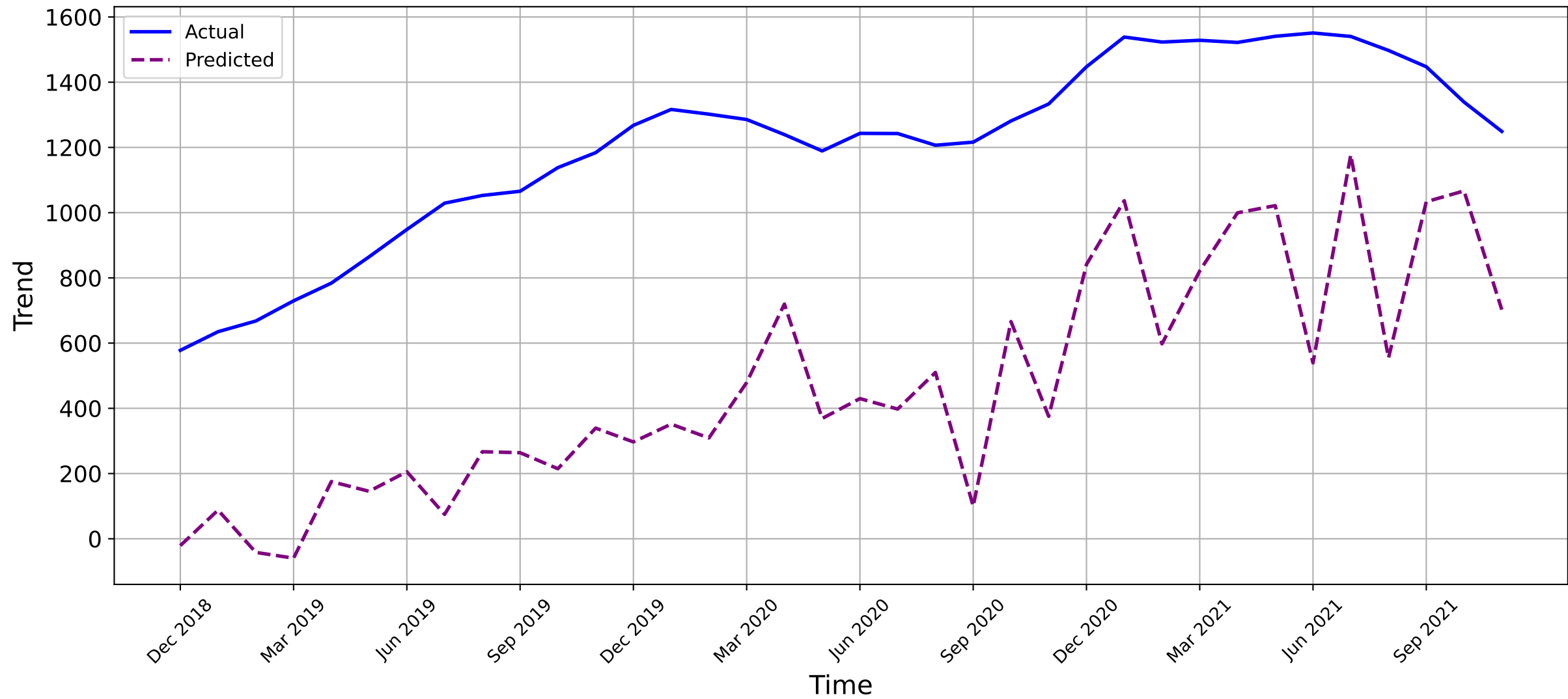
Solution_BLOCKCHAIN_Mentions - Validation
